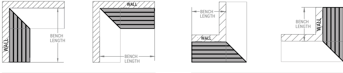
Inside Corner LY-A30-IN (shown) or LY-C30-IN
